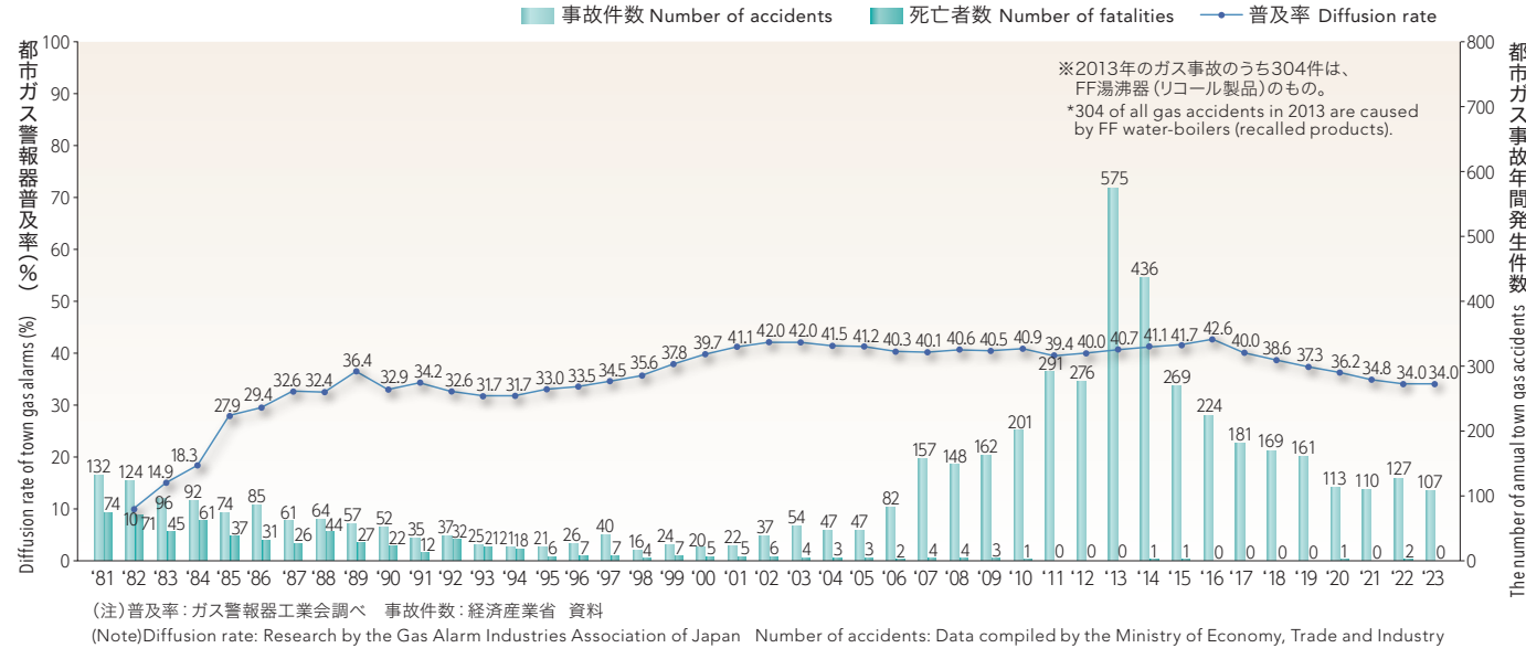
Diffusion Rate of Town Gas Alarms and the Number of Accidents – Diffusion rate remains at the 40% mark –
